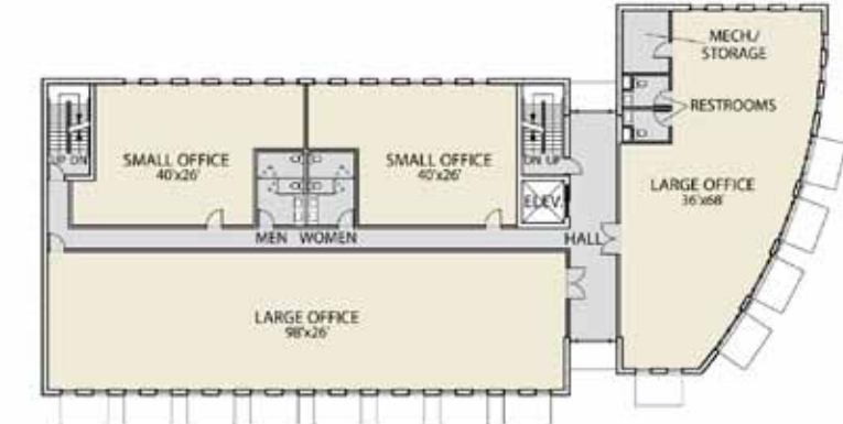
SECOND / THIRD FLOOR PLAN
